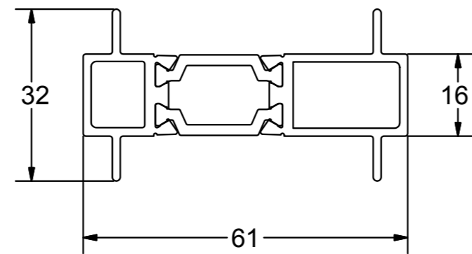
AW709 Concealed Coupling Bar (70mm)
