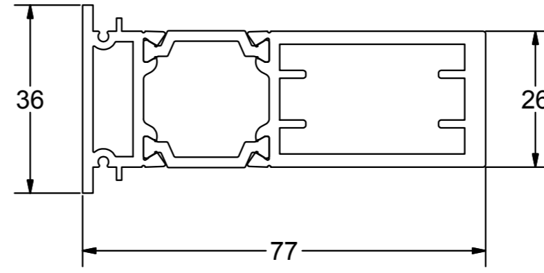
AW705 26mm Coupling Bar (70mm)
