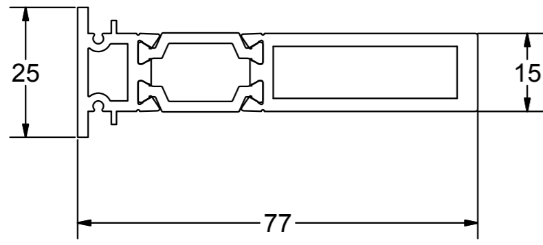
AW702 15mm Coupling Bar (70mm)
