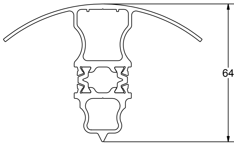
AW715 100-120° Bay Pole (70mm)
