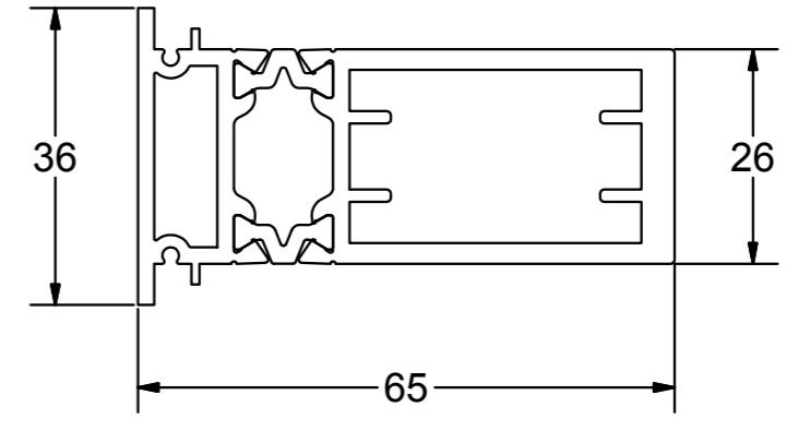
AW706 26mm Coupling Bar (58mm)
