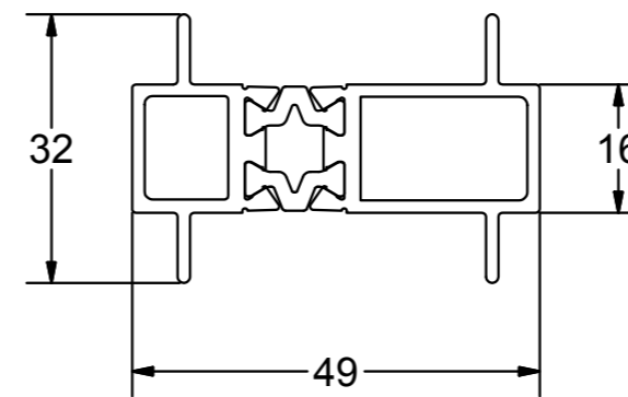
AW710 Concealed Coupling Bar (58mm)
