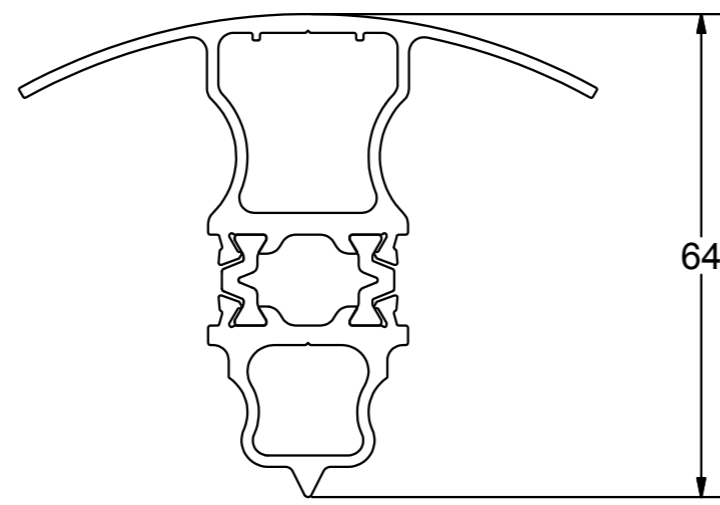
AW716 120-140° Bay Pole (70mm)
